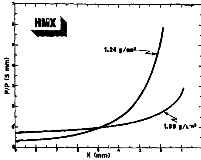
Fig. 6. Common-curve buildup for two densities of HMX.
