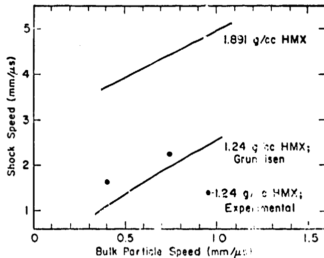
Fig. 1. Hugoniot data for HMX.
