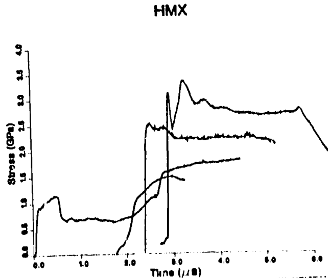
Fig. 5. In addition to profiles in Fig. 2, transmitted profiles for samples 3.1 and 4.0 mm thick are included. Run distance to detonation is 5.2 mm.
