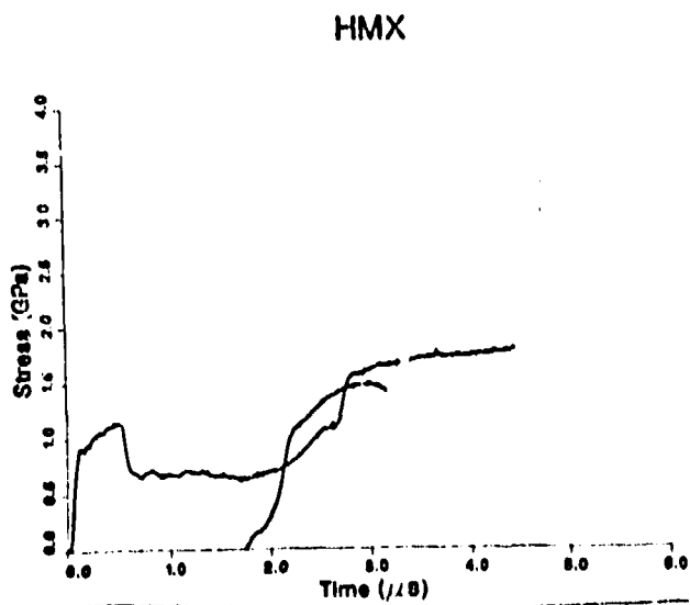
Fig. 4. Input and transmitted profiles for a 2.1-mm-thick sample of 1.24 g/cm 3 HMX.
