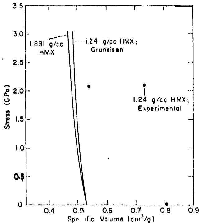
Fig. 2. P-V data for HMX.
